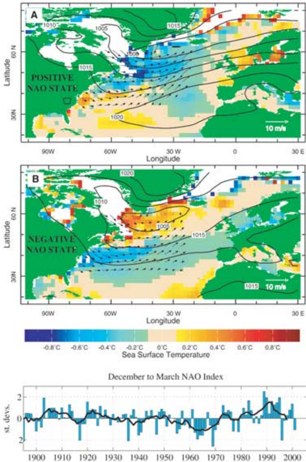
Figure 2. Schematic diagram depicting spatial characteristics of December–March positive (top panel) and negative (middle panel) phases of the North Atlantic Oscillation (NAO). Contours, vectors, and shading as in Figure 1. The bar graph in the (lower panel) depicts a time series of Hurrell’s December–March NAO index ( http://www.nao.html ). A 6-year running-average NAO index is shown with the solid curve. Composite fields are based on years in which the NAO index is either + or - one standard deviation from its mean value, otherwise as in Figure 1.
