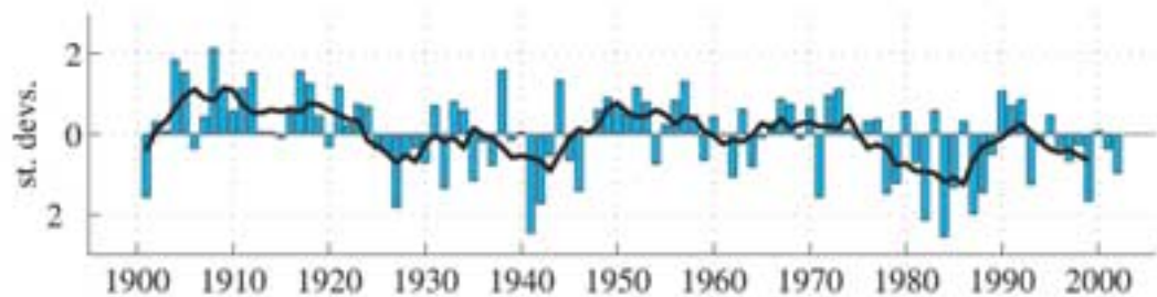
Figure 1. Composite diagram depicting spatial characteristics of November–March strong ( top panel ) and weak ( middle panel ) Aleutian Low conditions. Contours depict sea level pressures (in millibars), vectors indicate surface winds, and shading indicates SST anomalies. The bar graph in the lower panel depicts a time series of Hurrell’s November–March Aleutian Low index ( http://www.np.html ). A 6-year running-average AL index is shown with the solid curve. Composite fields are based on years in which the PNA index is either + or - one standard deviation from its mean value. Gridded data are from the NCEP/NCAR reanalysis data set (CDAS-1) for the period 1949–2001. Winds are at the 10-m level, SST is from the surface temperature data, which over the ice-free ocean are given by a blend of satellite and ship data.
